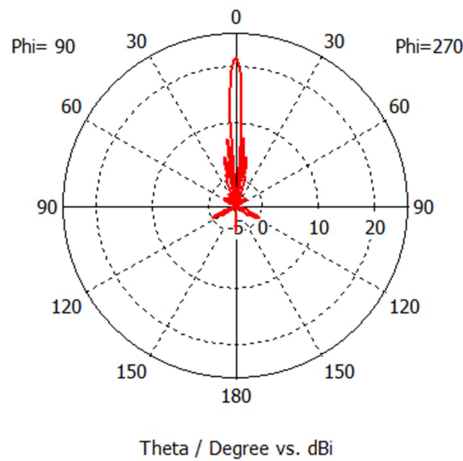
4200 МГц Farfield Realized Gain Abs (Phi=90)
