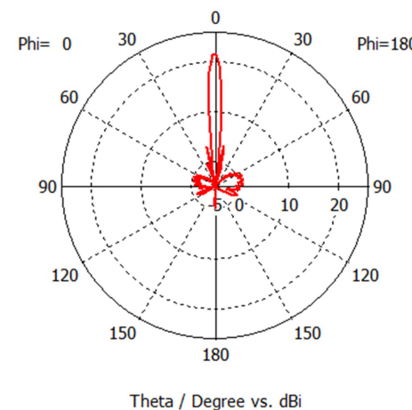
4200 МГц Farfield Realized Gain Abs (Phi=0)
